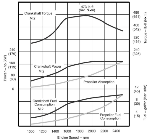
M2 PERFORMANCE CURVE
